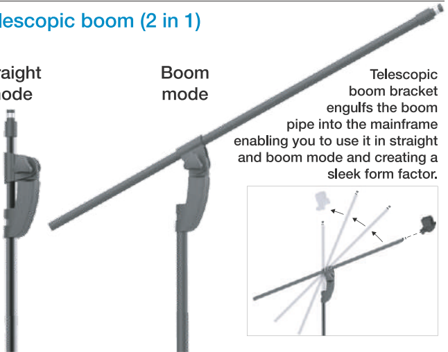
★ MT24 NEW Mic Stand Floor stand w/collapsible base
